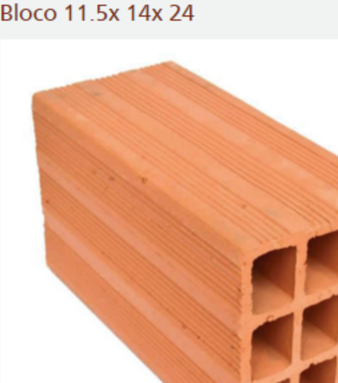
Bloco 11.5x14x24
